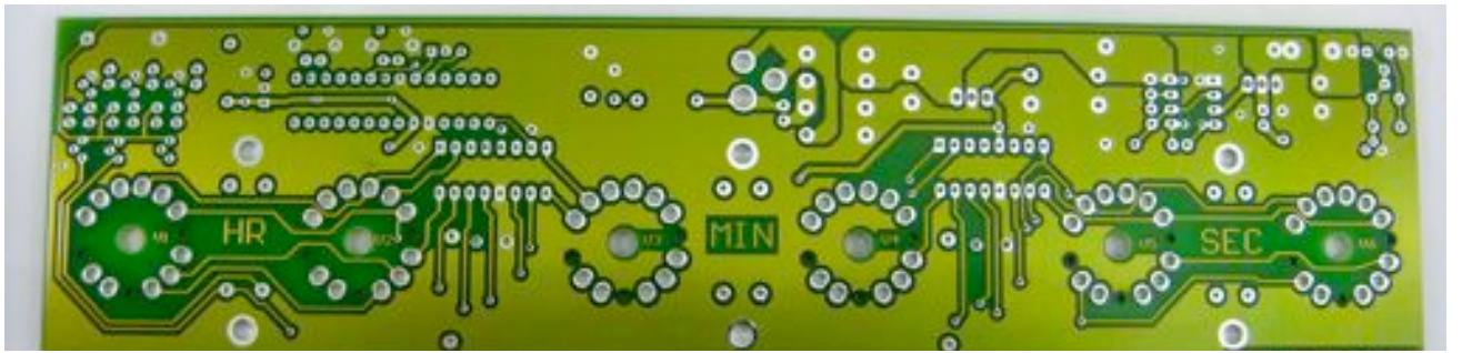
Figure 2: Solder Side
