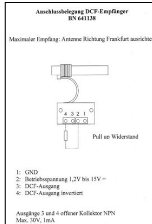
The Conrad DCF77 module
