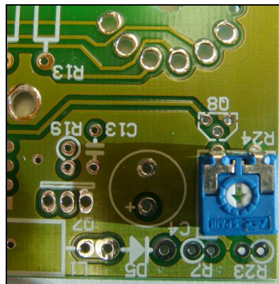
This trimmer is used to adjust the voltage to 180V DC later.
